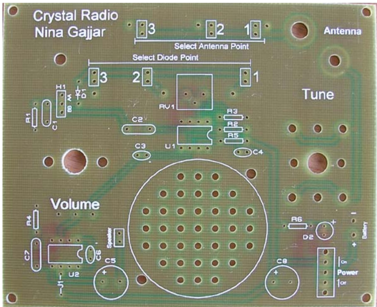
PCB Picture: Front Side
